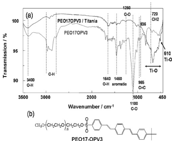
Figure 4. (a) FT-IR spectra of amphiphilic PEO 17 -OPV 3 molecule and its hybrid with titania. (b) Chemical structure of PEO 17 -OPV 3 molecule.
