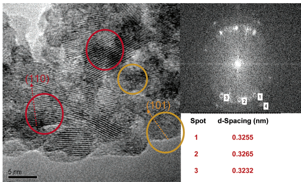
Figure 6. HR-TEM micrograph and the corresponding FFT pattern of PEO 17 -OPV 3 -templated TiO 2 nano-hollow rod.
