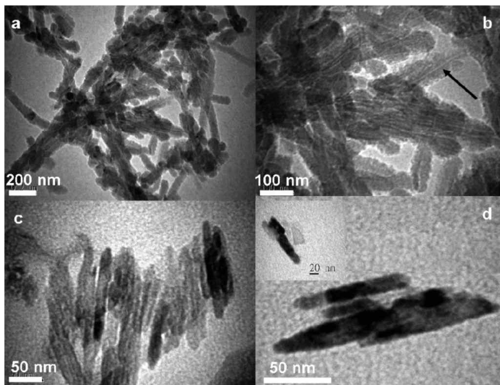
Figure 2. TEM micrographs of PEO 17 -OPV 3 -templated TiO 2 nano-hollow rods (a and b are unstained samples, c and d are RuO 4 -stained samples).
