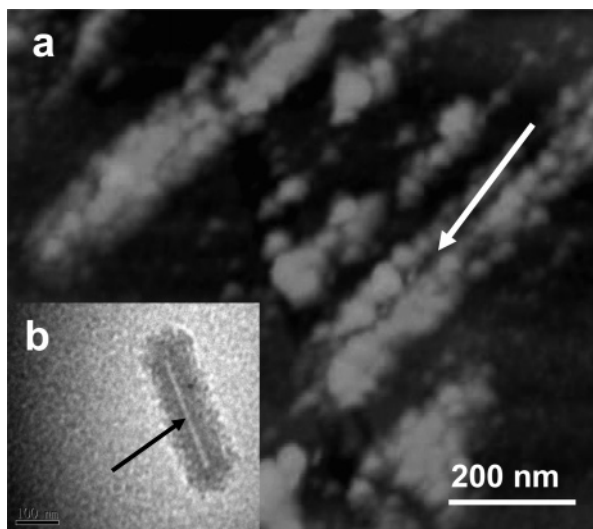
Figure 3. (a) AFM image of templated TiO 2 nano-hollow rods on mica and (b) their TEM image.
