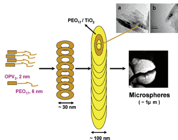
Figure 5. Illustration of assembly mechanism.
