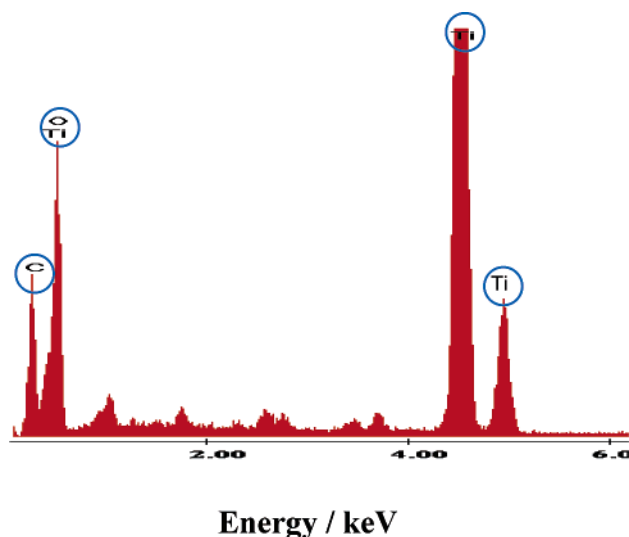
Figure 7. EDX analysis of PEO 17 -OPV 3 -templated TiO 2 nano-hollow rod.
